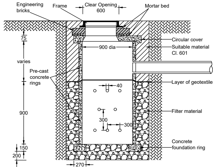
Pre-cast Concrete Soakaway
