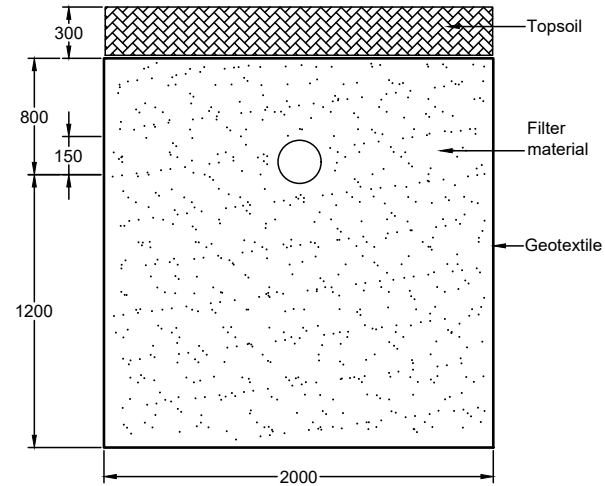
Trench Soakaway
