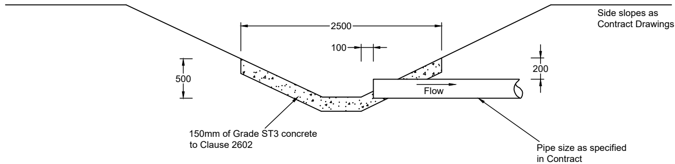
Section
