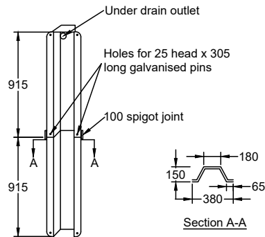
Headwall Detail
