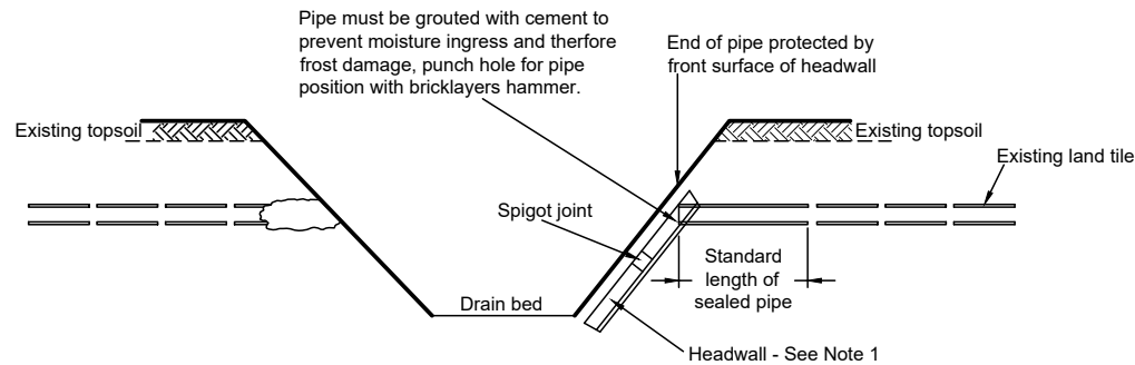
Land Drain Intercepted by Ditch
