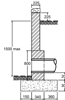
Section (for retained height up to 1.5m)
