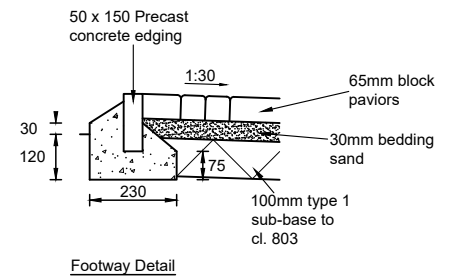
Footway Detail
